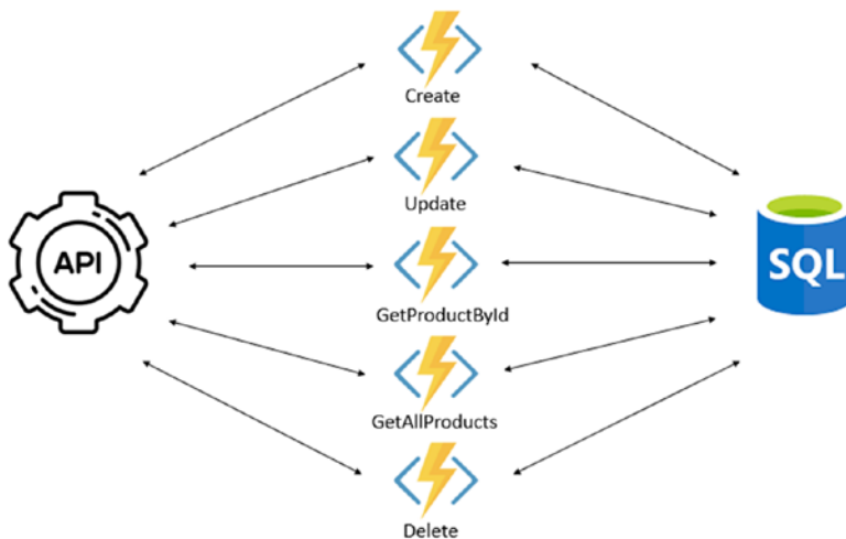
Figure 8-1. Architecture diagram of the proof of concept
