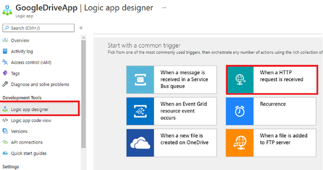
Figure 19-25. Click “When a HTTP request is received”
