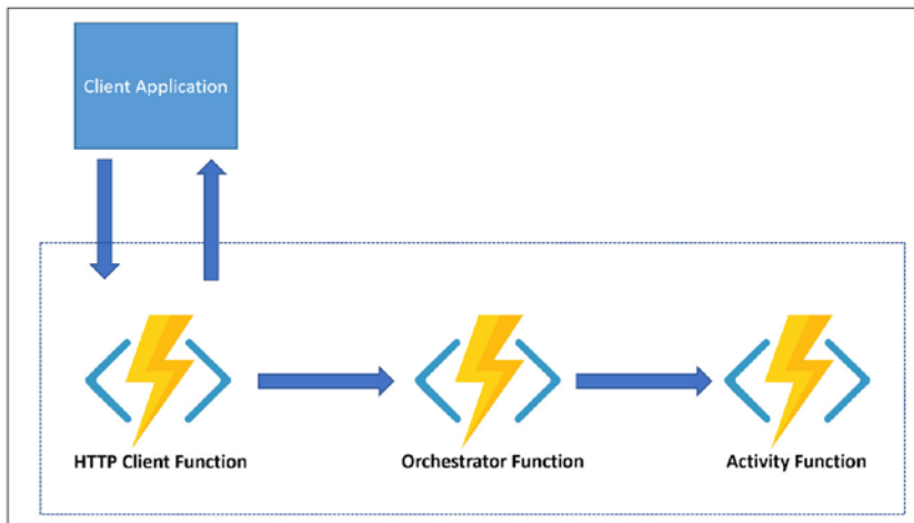
Figure 18-4. Async HTTP pattern
