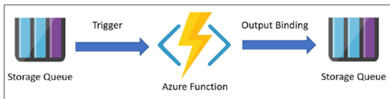
Figure 3-2. Azure function triggered by a Queue Storage
