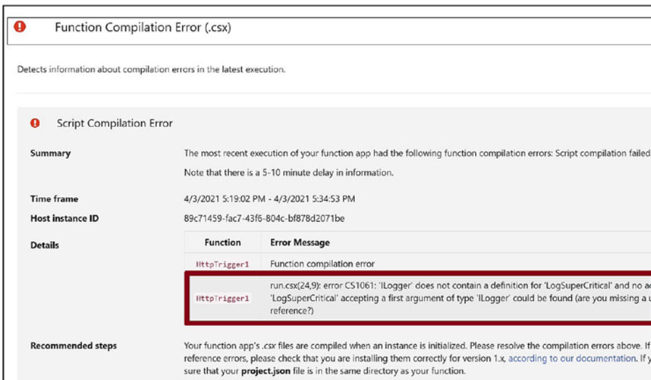
Figure 10-18. Function compilation error
