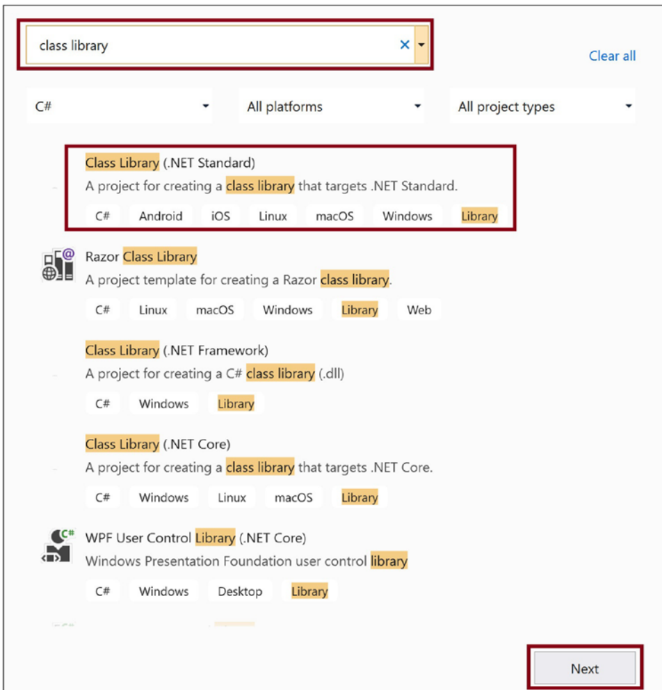
Figure 7-7. Set the type of project as Class Library (.NET Standard)
