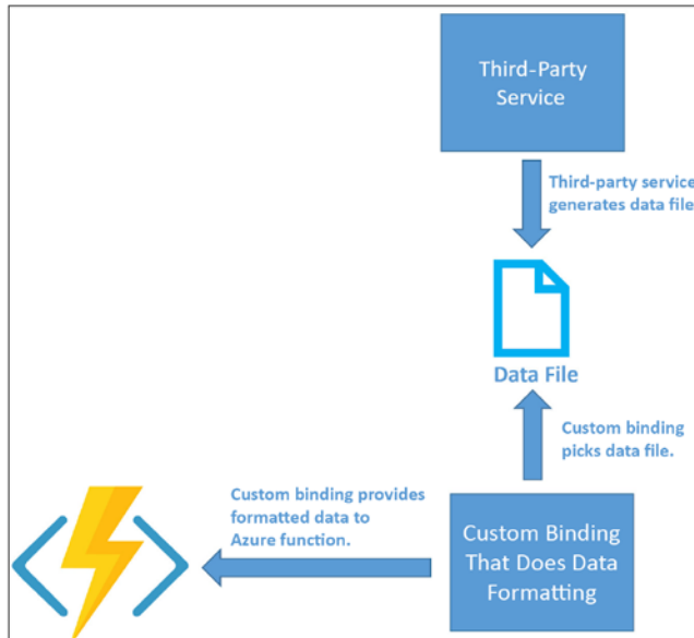
Figure 7-1. Custom binding scenario
