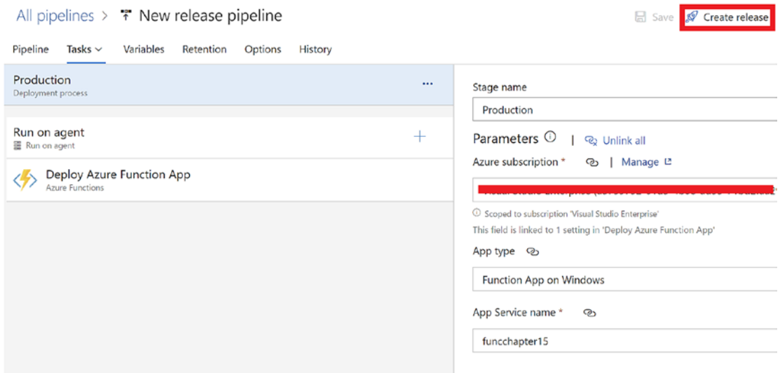
Figure 15-23. Click “Create release”
