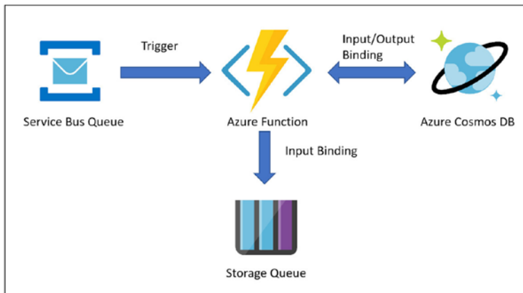
Figure 3-1. Triggers and bindings with Azure Functions
