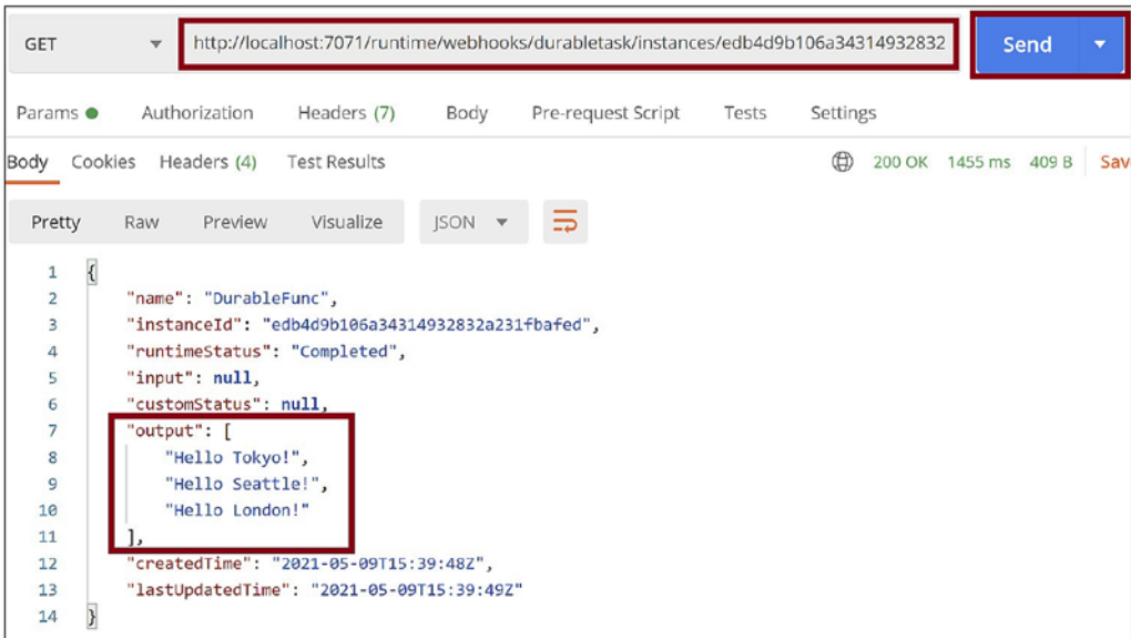
Figure 18-14. Azure Durable Functions workflow response
