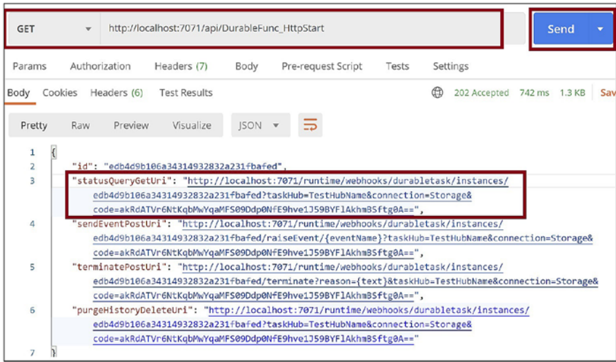
Figure 18-13. Invoke orchestrator client URL in Postman
