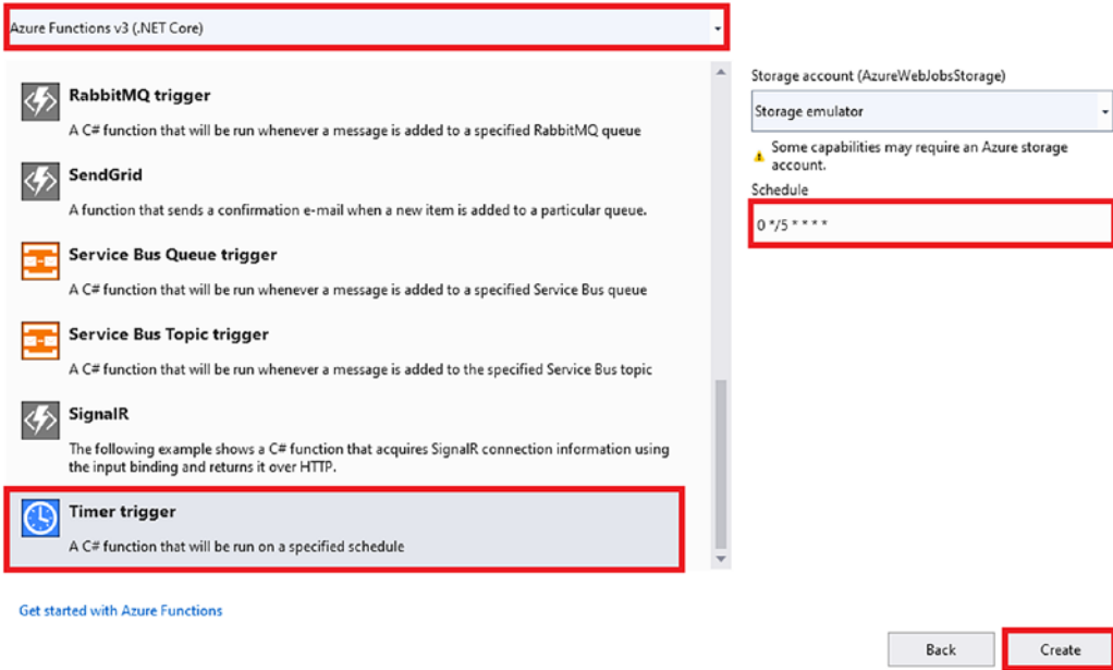
Figure 17-17. Select "Timer trigger" and Azure Function V3
