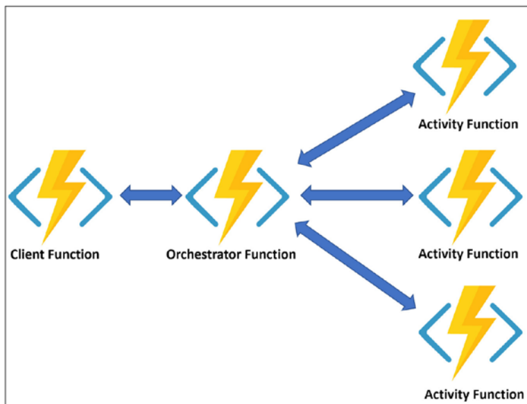
Figure 18-1. Azure Durable Functions components
