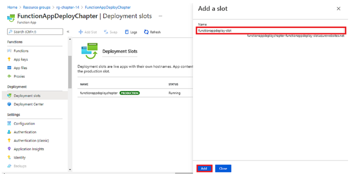
Figure 14-18. Click Add
