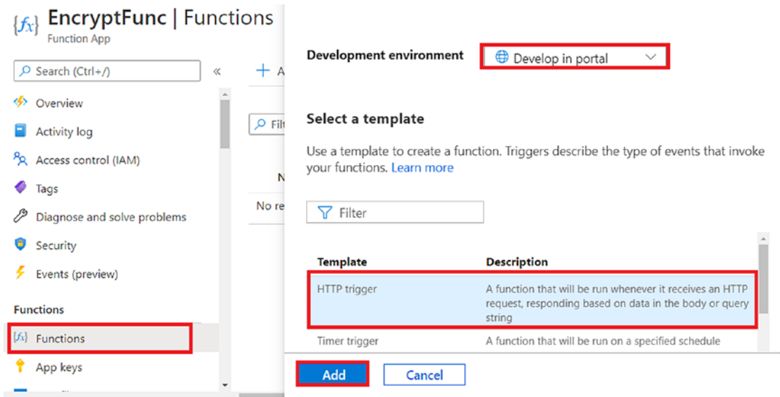
Figure 19-19. Click Add
