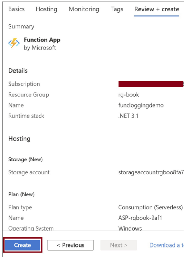
Figure 10-5. Click Create
