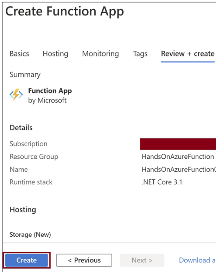
Figure 2-8. Click Create
