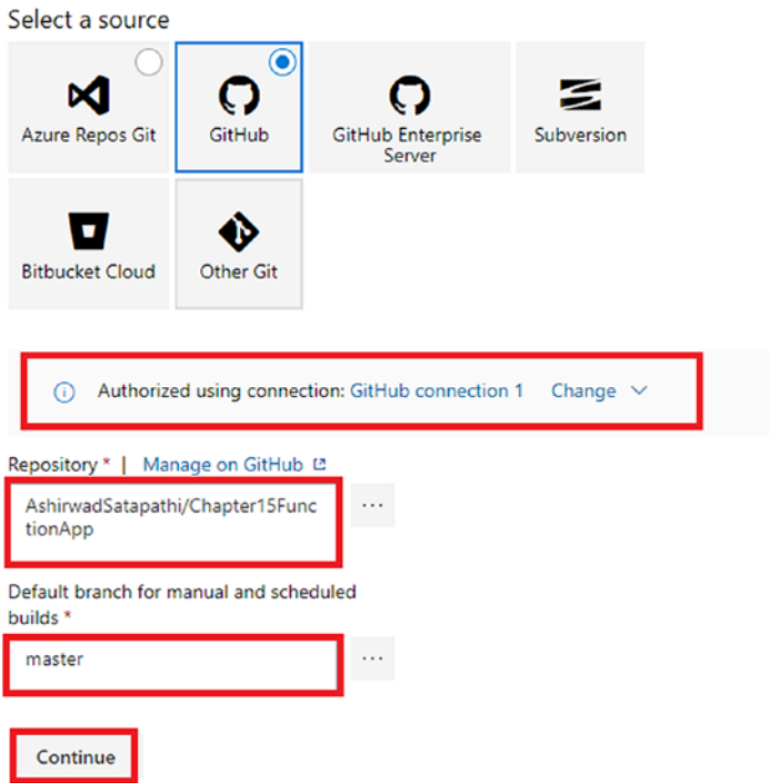
Figure 15-8. Click Continue
