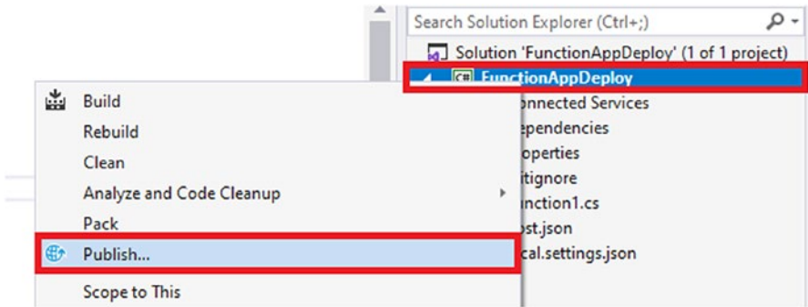
Figure 14-20. Click Publish
