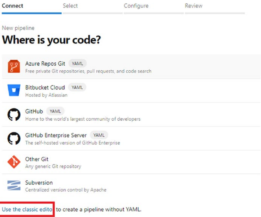
Figure 15-5. Click “Use the classic editor”
