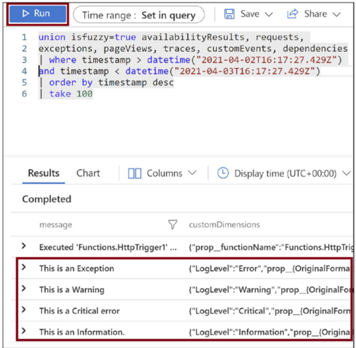
Figure 10-12. Run the query to get the logs
