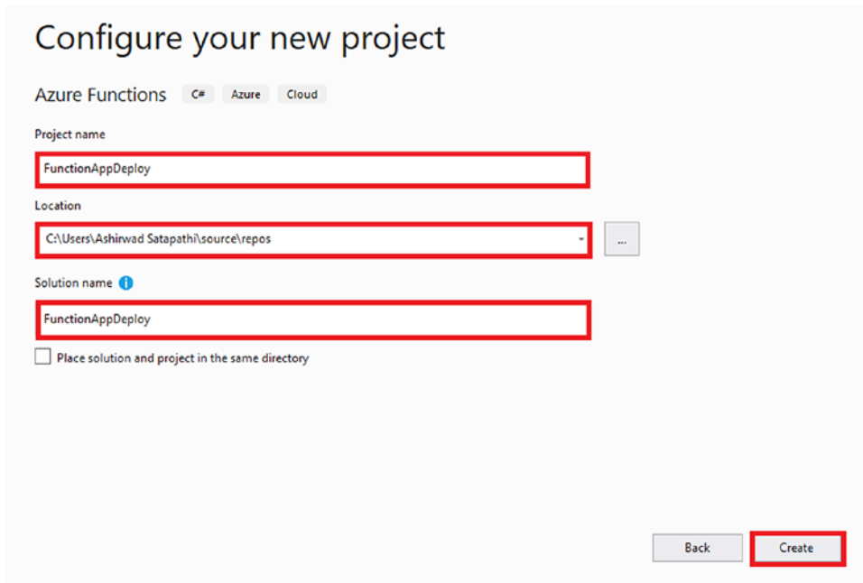
Figure 14-3. Click Create
