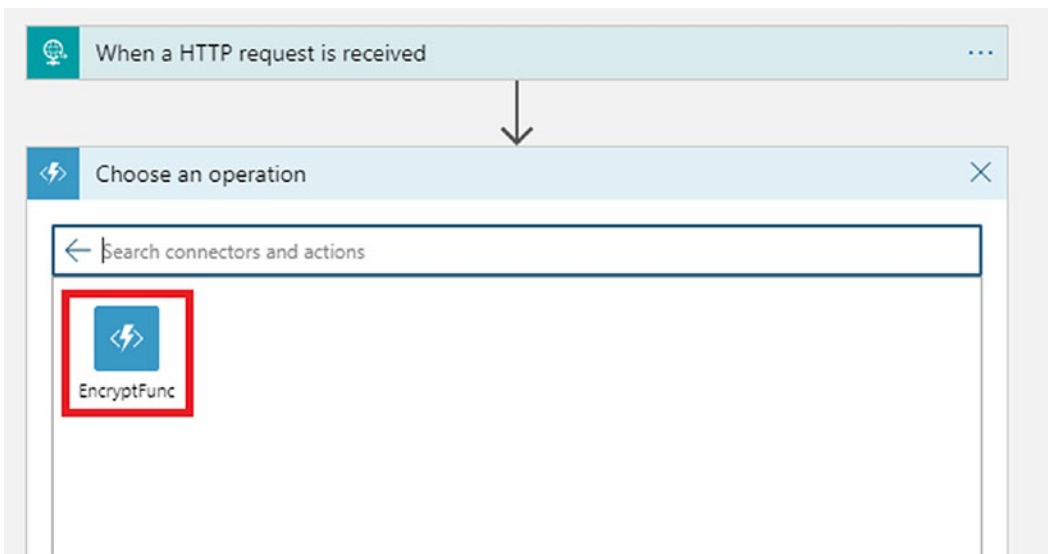
Figure 19-30. Click EncryptFunc
