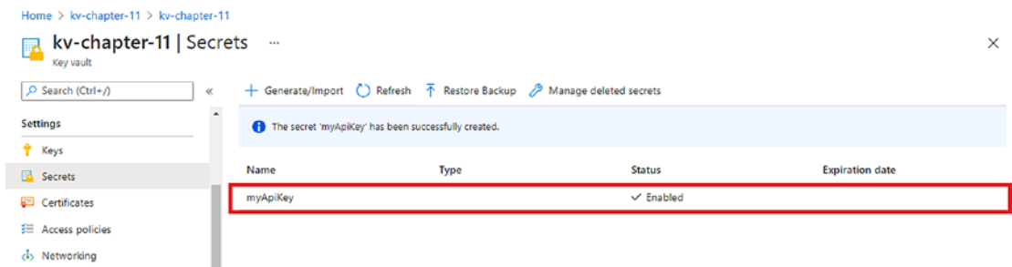
Figure 11-11. Click myApiKey
