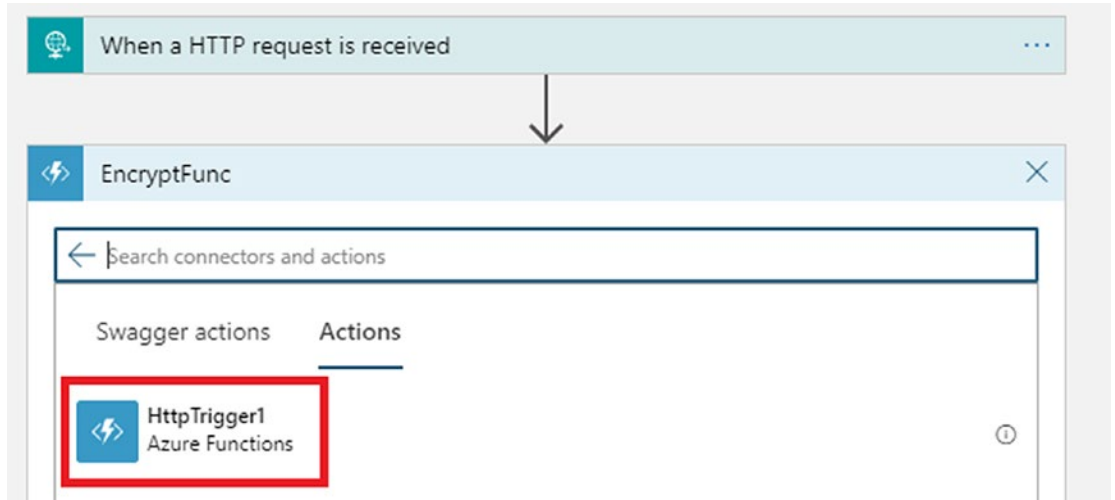
Figure 19-31. Click HttpTrigger1
