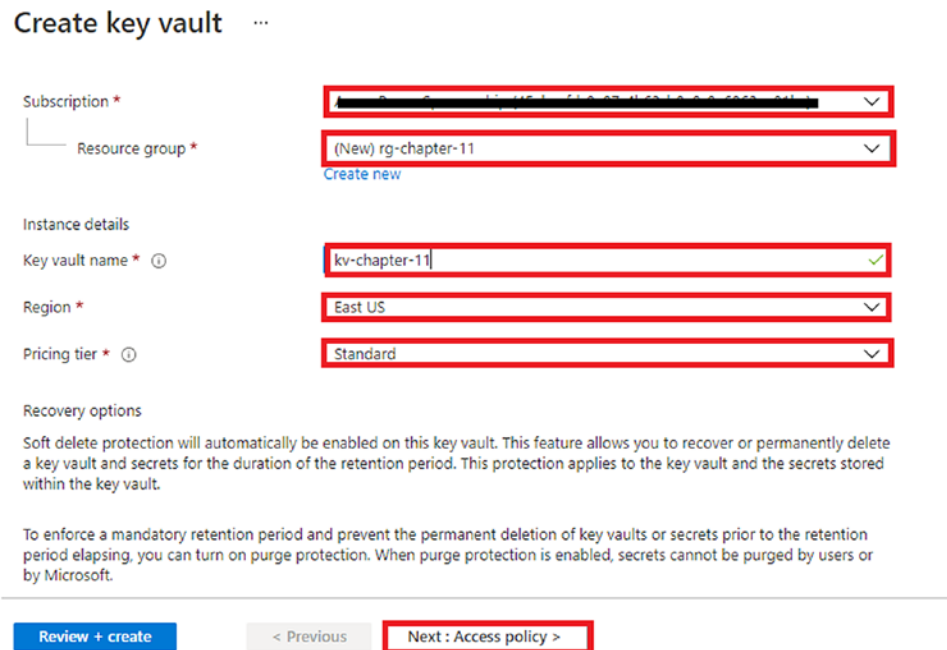
Figure 11-3. Click “Next: Access policy”
