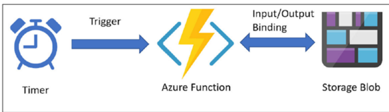
Figure 3-3. Azure function triggered by a timer
