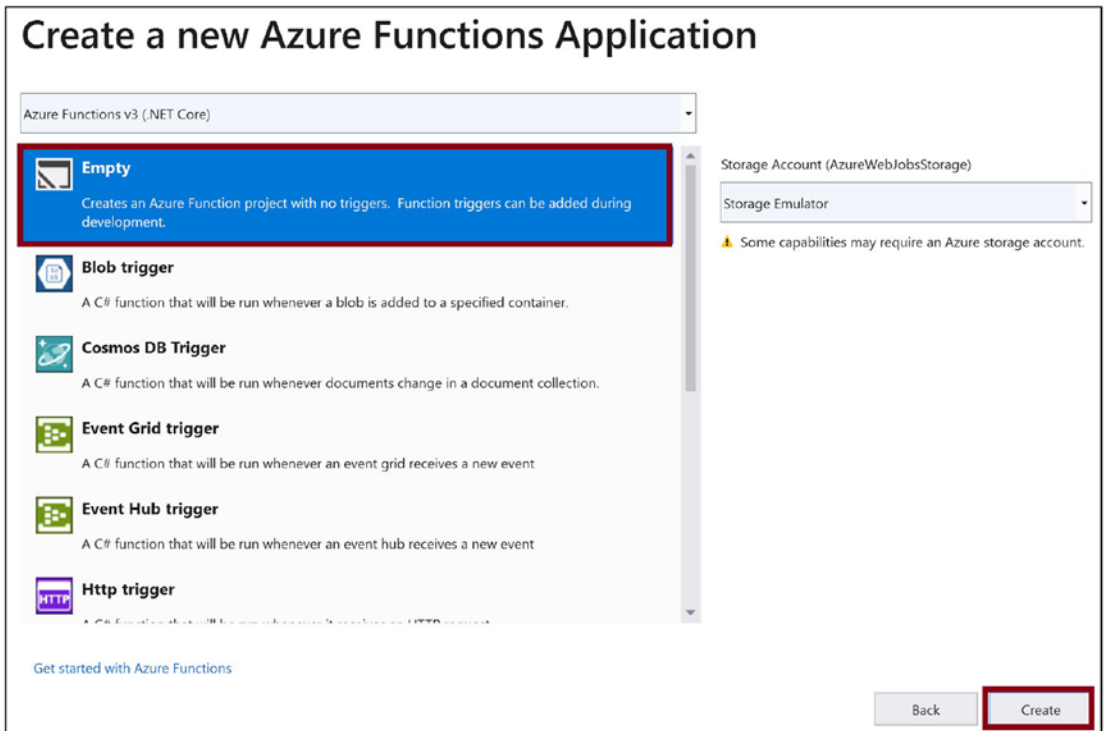
Figure 18-8. Select Empty
