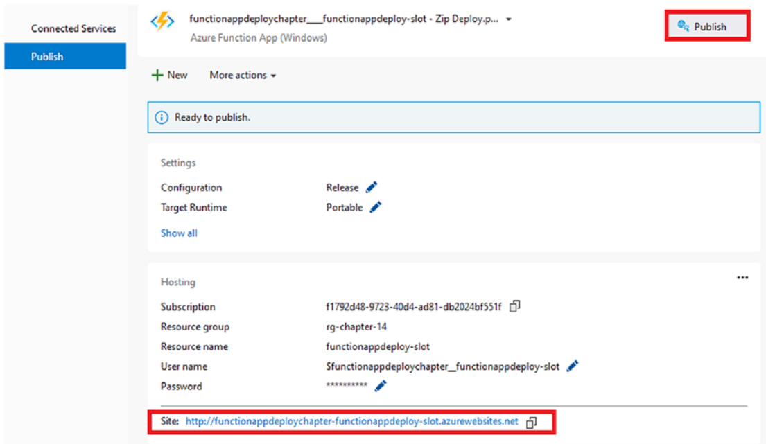
Figure 14-25. Click Publish
