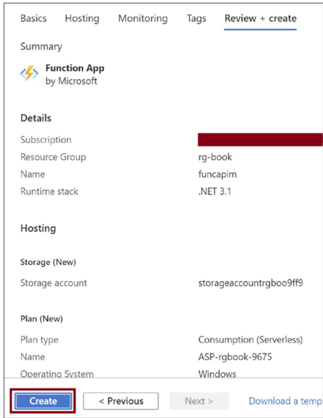
Figure 13-4. Click Create
