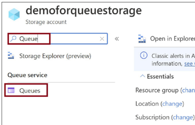
Figure 4-6. Click Queues
