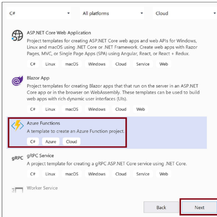
Figure 9-12. Click Next
