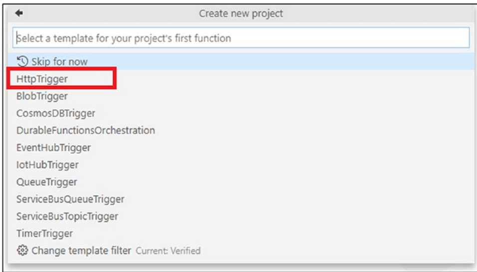
Figure 2-25. Select HttpTrigger
