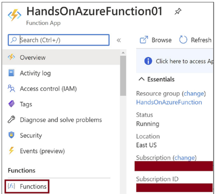
Figure 2-10. Click Functions
