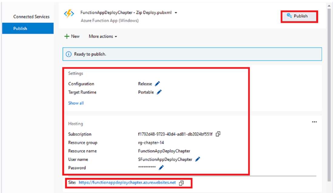
Figure 14-12. Click Publish
