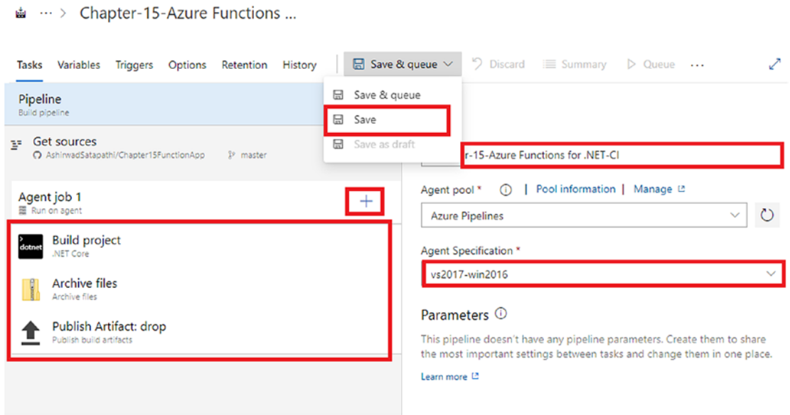
Figure 15-10. Click Save
