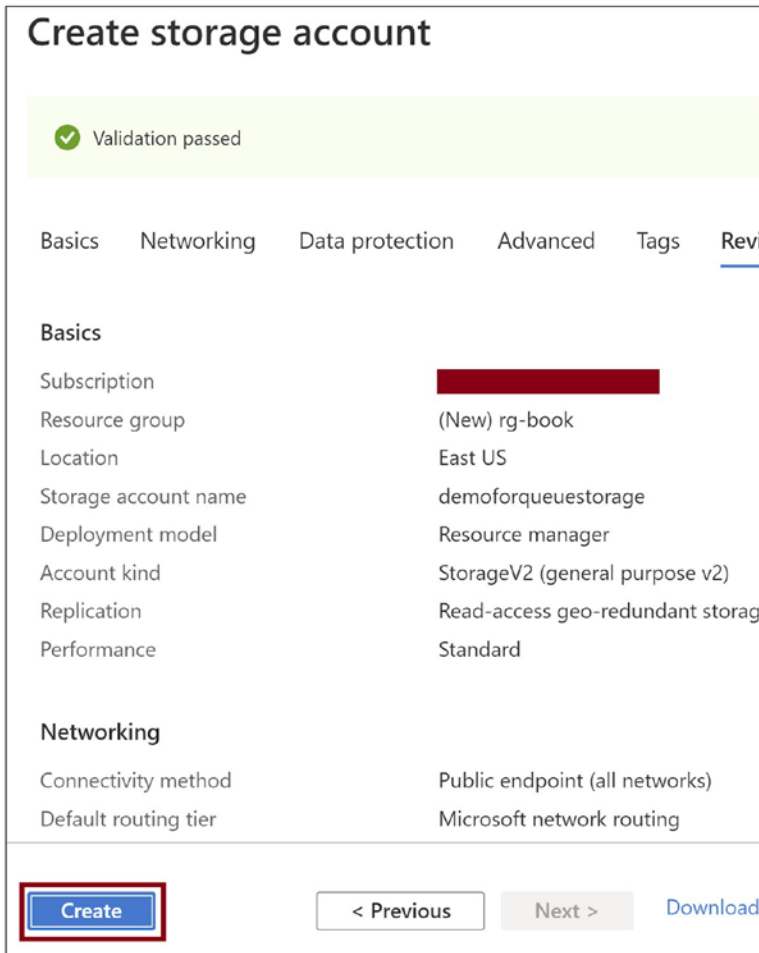
Figure 4-5. Click Create
