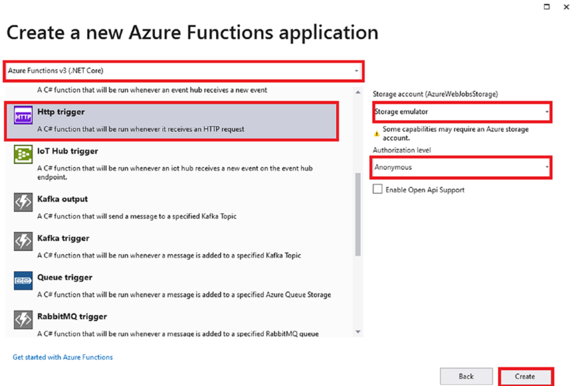
Figure 8-11. Select the trigger type and authentication level
