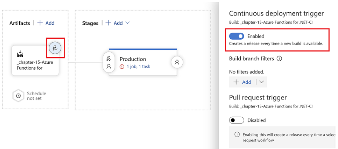
Figure 15-20. Enable a continuous deployment trigger
