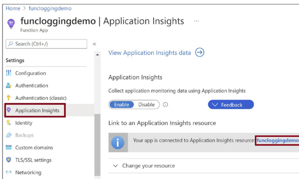
Figure 10-10. Go to the Application Insights resource
