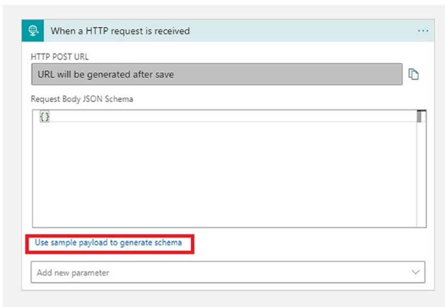
Figure 19-26. Click “Use sample payload to generate schema”
