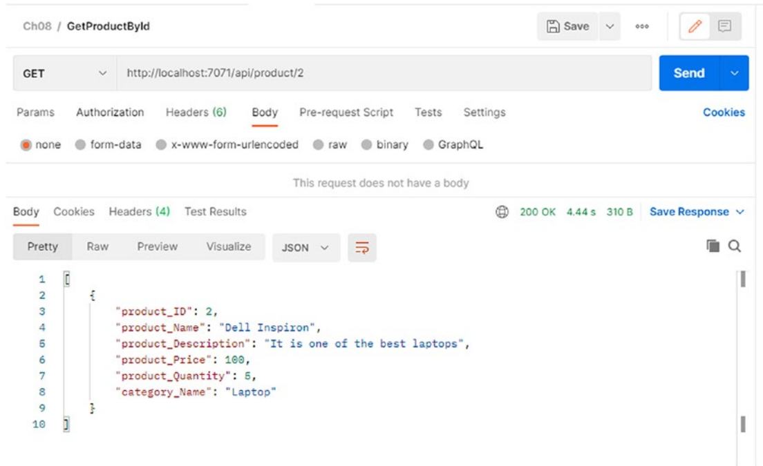
Figure 8-19. Response from the GetProductById function
