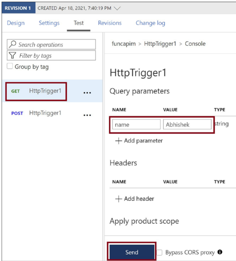
Figure 13-23. Provide the query parameter in the request
