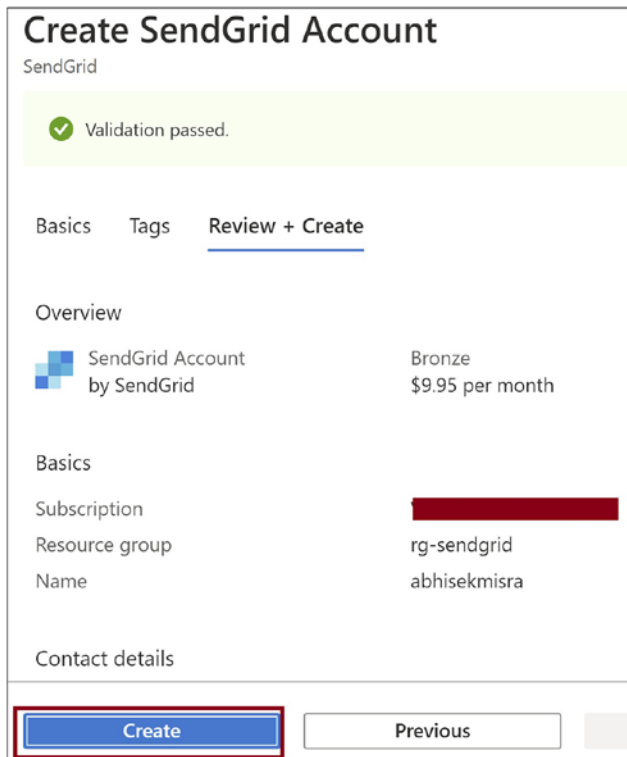
Figure 4-23. Click Create
