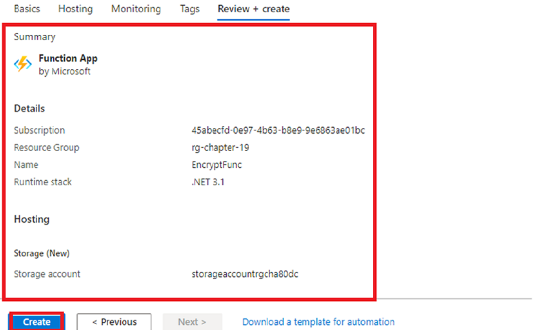
Figure 19-17. Click Create
