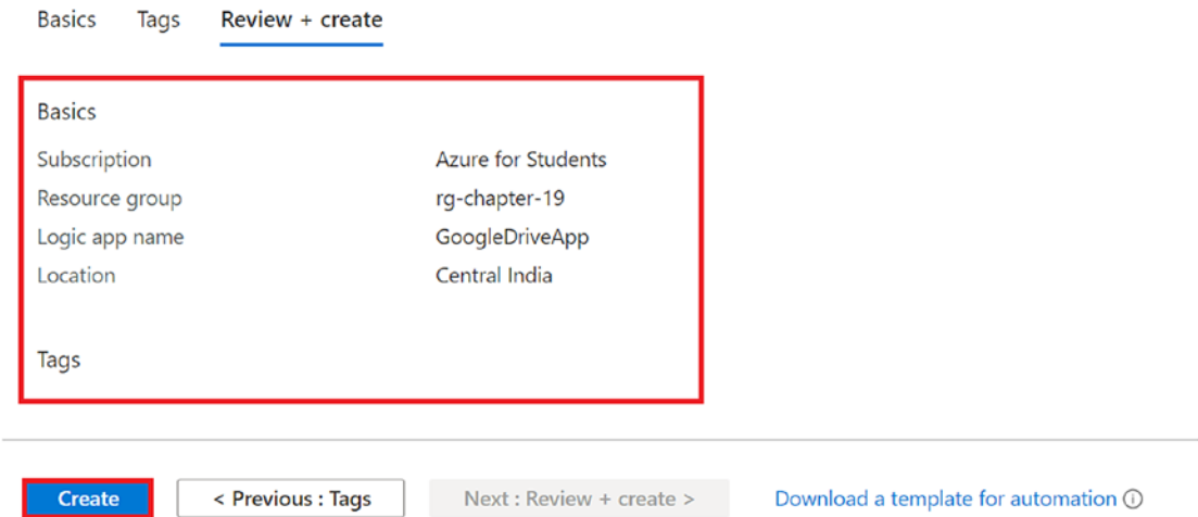
Figure 19-23. Click Create
