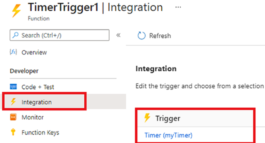
Figure 5-12. Click Integration
