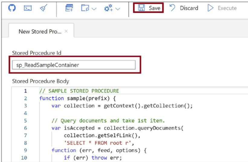
Figure 9-25. Save the stored procedure
