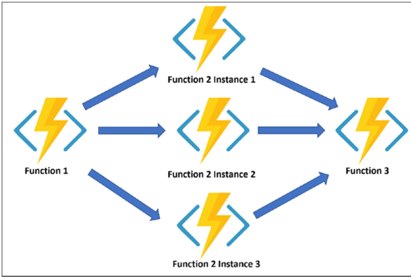
Figure 18-2. Fan-out and fan-in pattern
